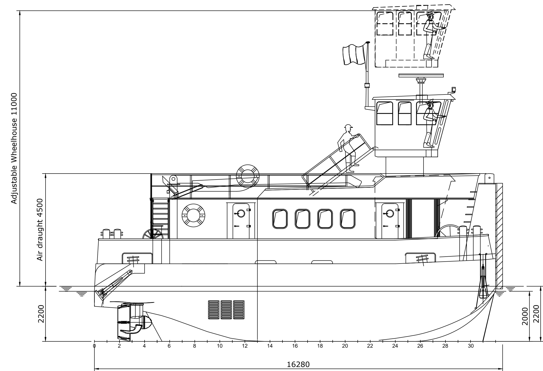
Side View
