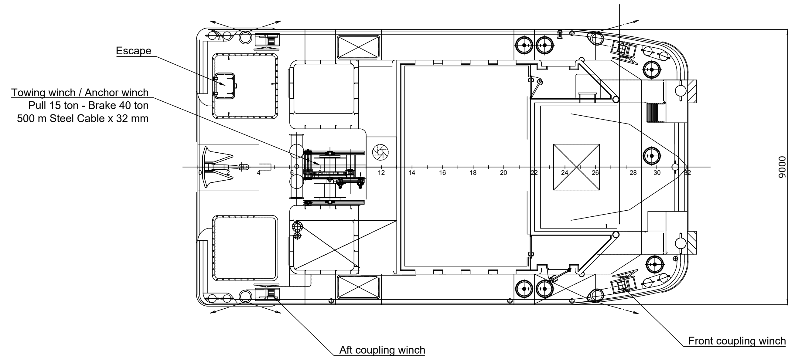
Top View
